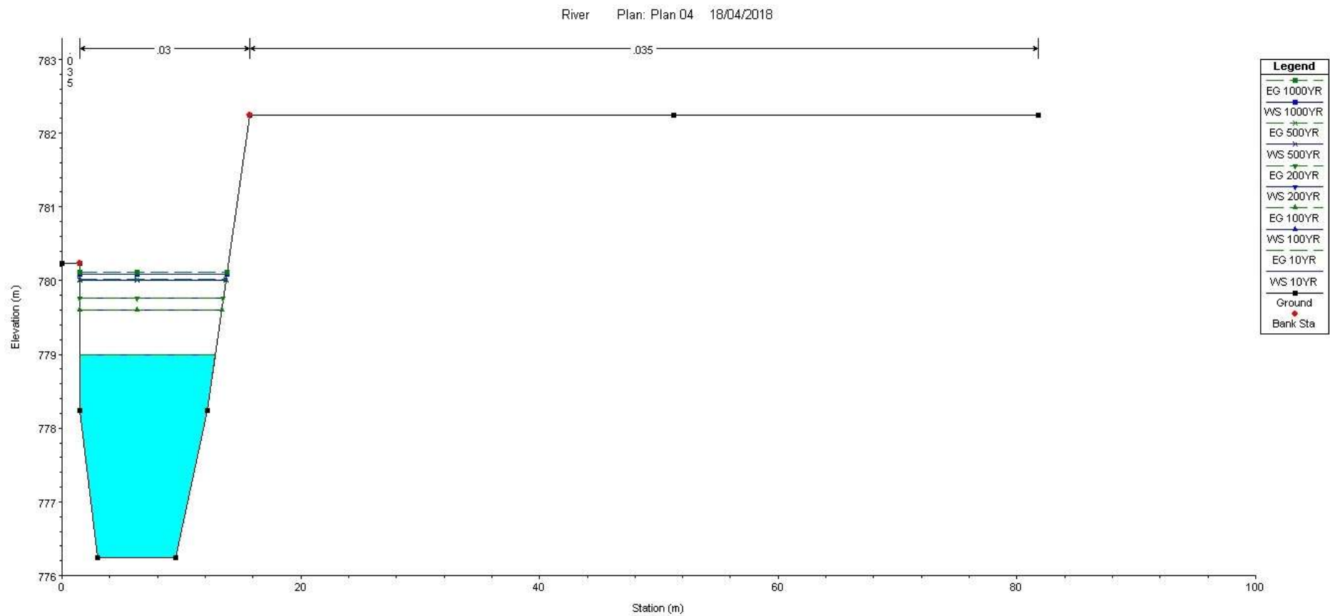
Figure 5-2: Water level elevations (m) at cross-section 16 (Chainage 477.6417) for the 10% AEP, 1% AEP, 0.5% AEP, 0.2% AEP and 0.1% AEP events.
