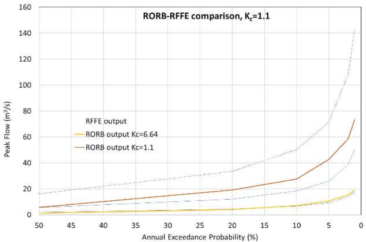
Figure B-4: RFFE – RORB calibration for the study catchment (Top panel, K_c = 6.64 and bottom panel, K_c = 1.1 )
