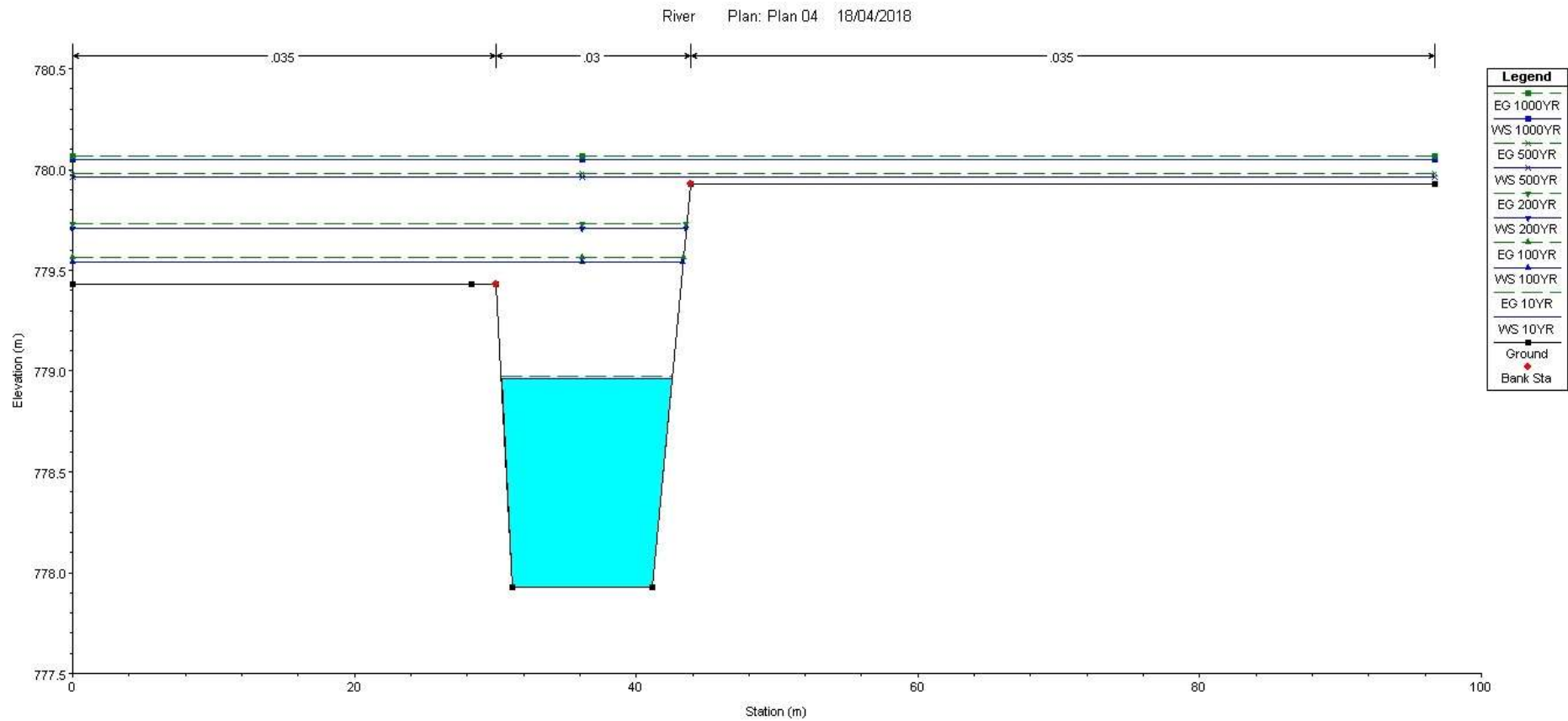
Figure 5-4: Water level elevations (m) at cross-section 7 (Chainage 210.2481) for the 10% AEP, 1% AEP, 0.5% AEP, 0.2% AEP and 0.1% AEP events.
