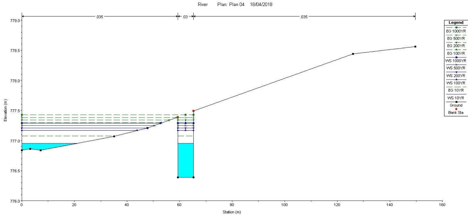
Figure 5-6: Water level elevations (m) at cross-section 1 (Chainage 1.4864) for the 10% AEP, 1% AEP, 0.5% AEP, 0.2% AEP and 0.1% AEP events. Noting that the water on the left hand side of the cross section is an artefact of modelling and that the flow would be contained within the cross section.
