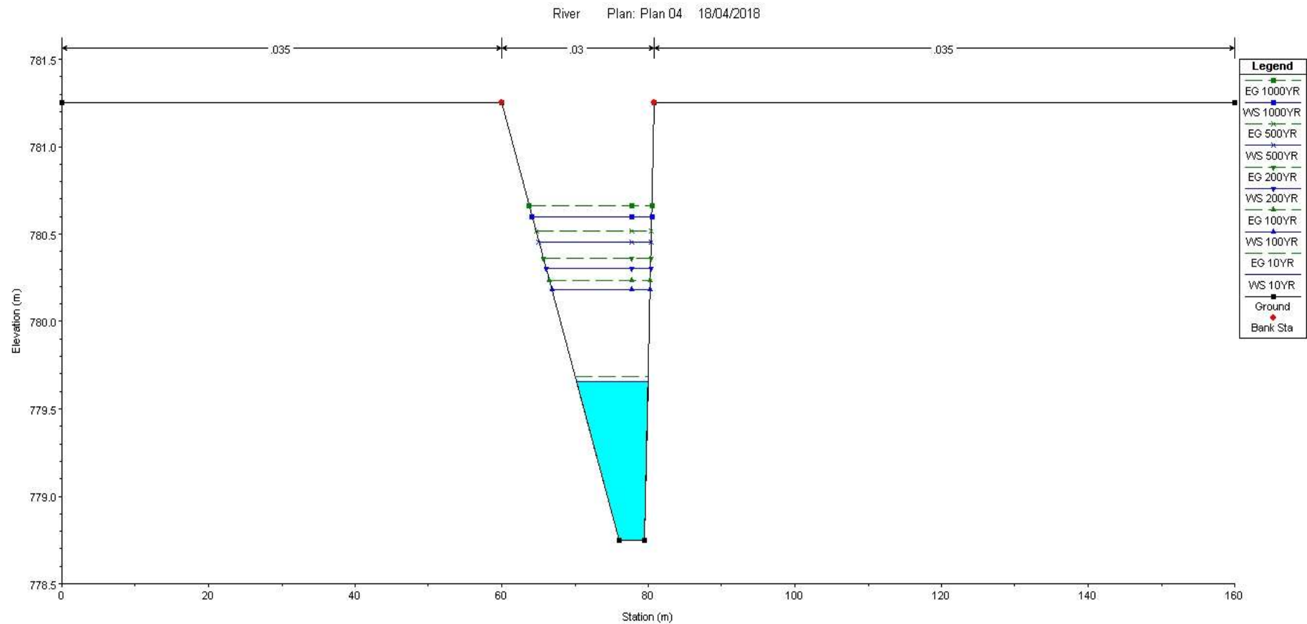
Figure 5-1: Water level elevations (m) at cross-section 20 (Chainage 602.9097) for the 10% AEP, 1% AEP, 0.5% AEP, 0.2% AEP and 0.1% AEP events 5 .
