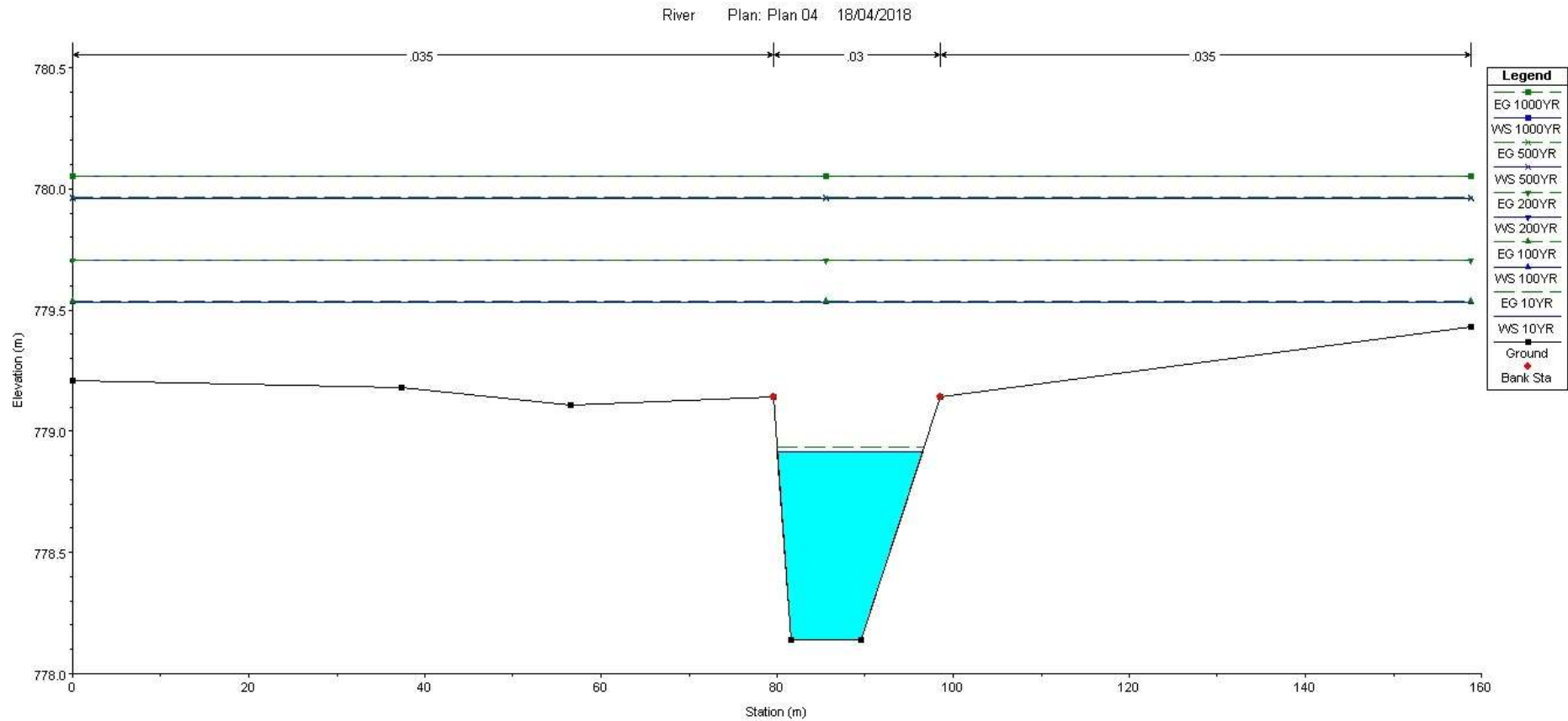
Figure 5-5: Water level elevations (m) at cross-section 4 (Chainage 110.5611) for the 10% AEP, 1% AEP, 0.5% AEP, 0.2% AEP and 0.1% AEP events.
