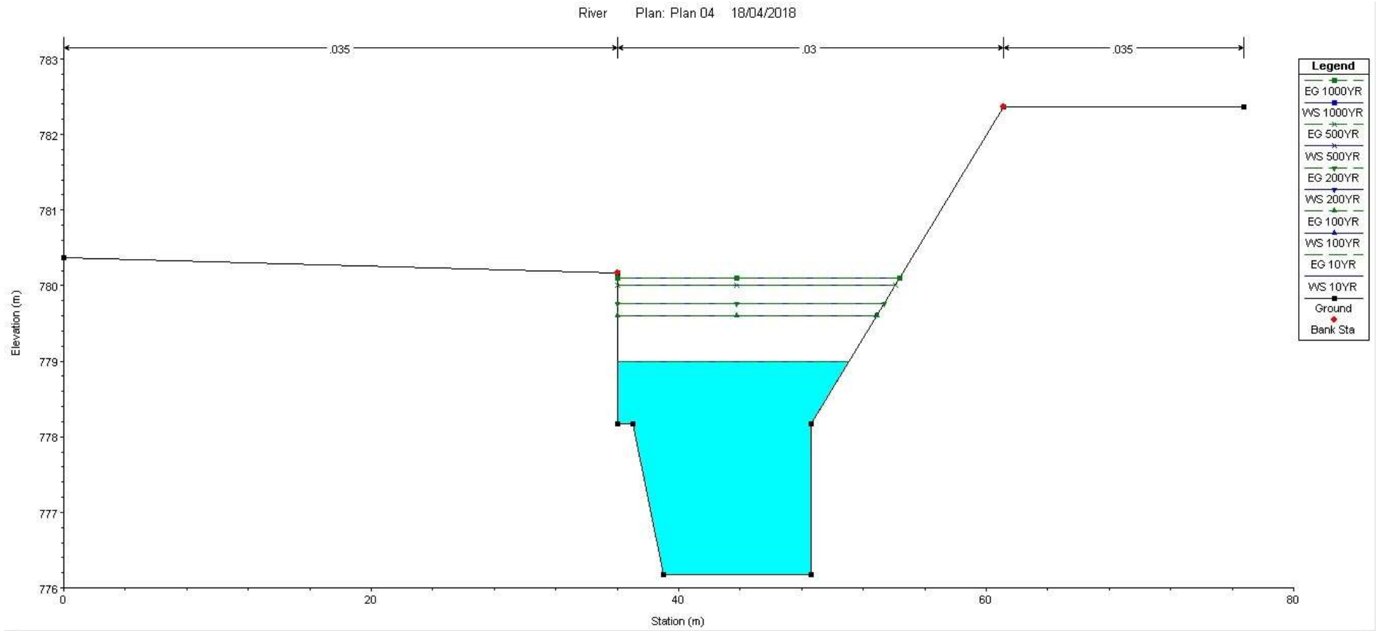
Figure 5-3: Water level elevations (m) at cross-section 13 (Chainage 423.6517) for the 10% AEP, 1% AEP, 0.5% AEP, 0.2% AEP and 0.1% AEP events.
