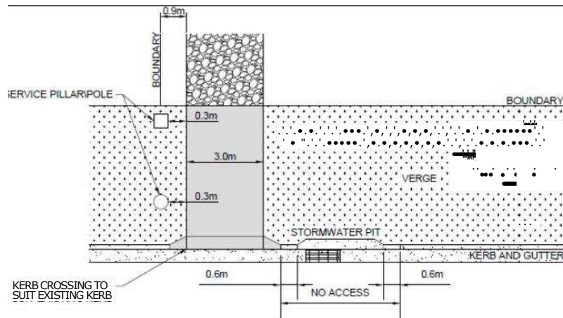
DETAIL A - MINIMUM CLEARANCE TO SURFACE UTILITY STRUCTURES
