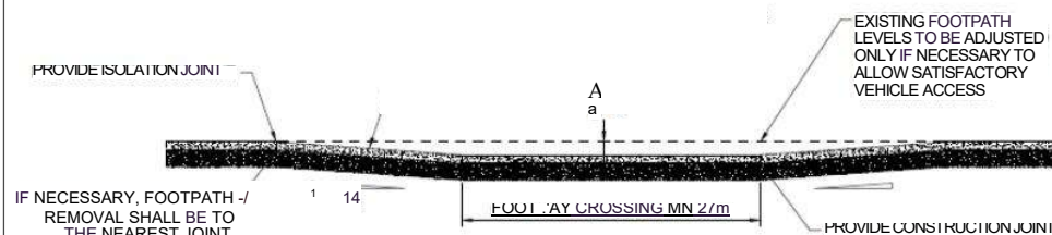
SECTION ALONG FOOTPATH (PATHS >1.5m SHALL NOT BE ADJUSTED)
