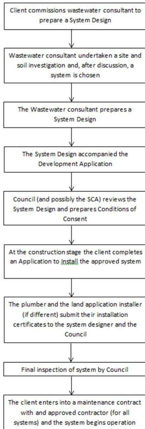
Figure 10 Flowchart to design and install an on-site wastewater systems
