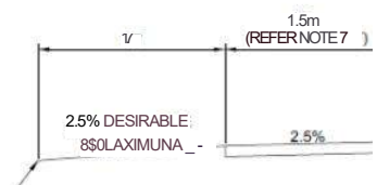
PROFILE OF FOOTWAY CROSSING (PATHS >1.5m SHALL NOT BE ADJUSTED)
